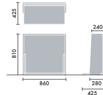
Utility cart for concealing under-counter storage
